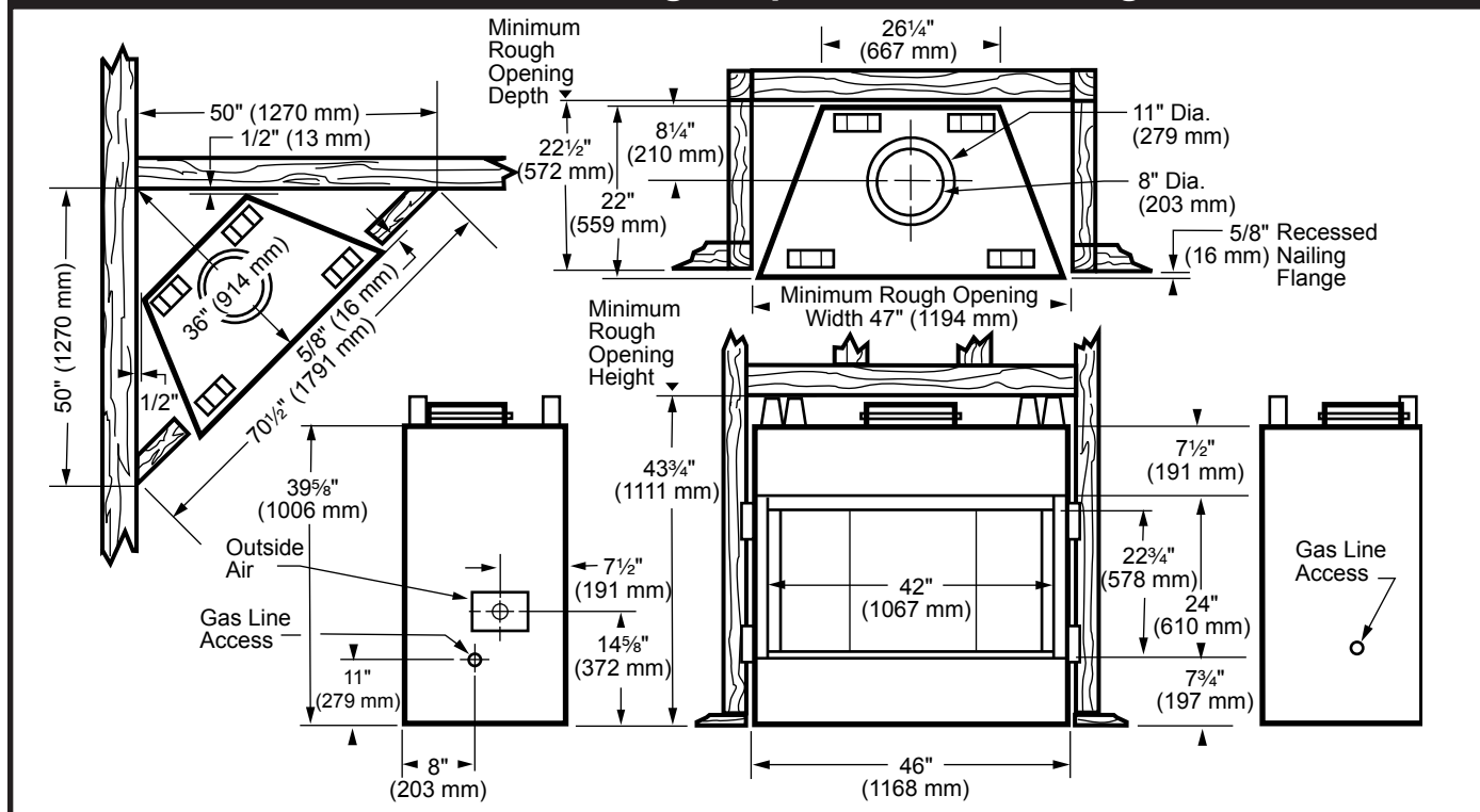
Fig. 2 ODSR42A specifications and framing.
