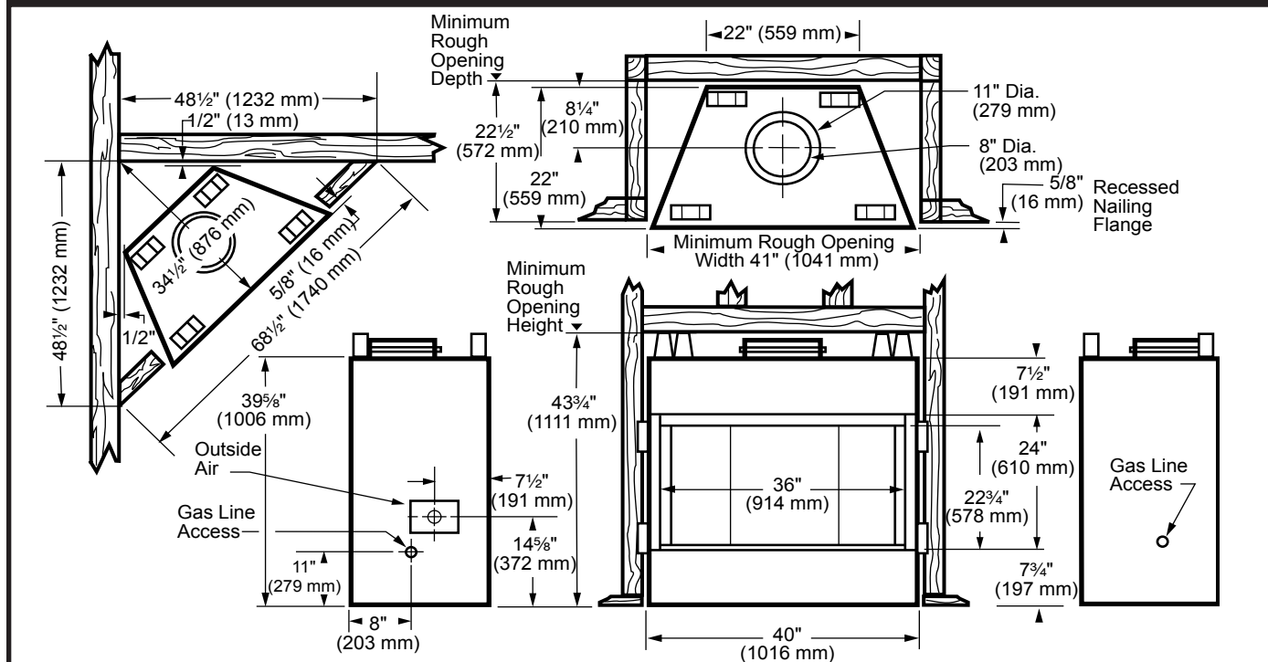
Fig. 1 ODSR36A specifications and framing.
