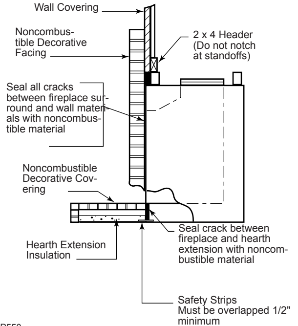
Fig. 26 Sealing gaps.
