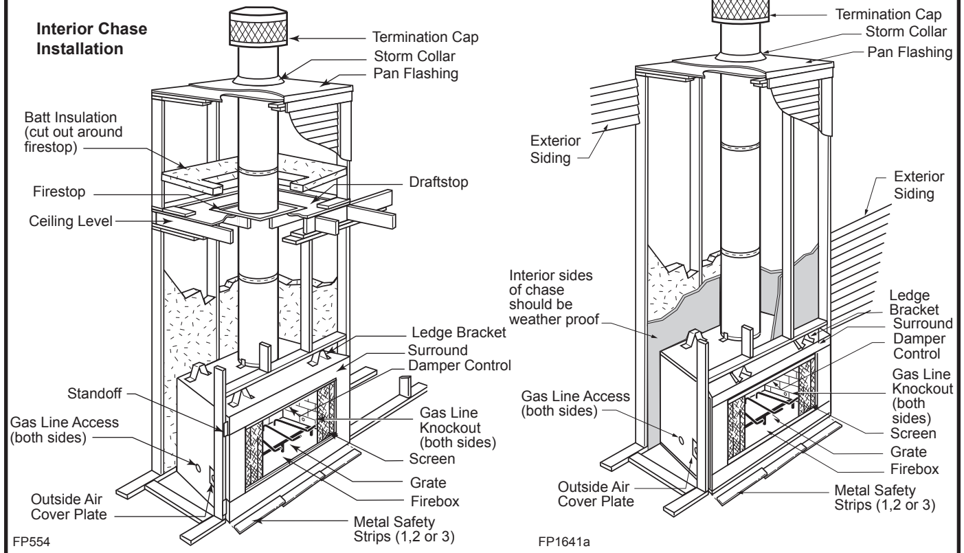
Fig. 5 Fireplace and chase parts identification.
